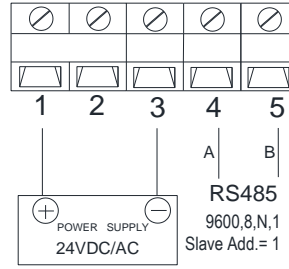
RS485/Modbus
