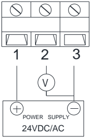
0~10V/5V
